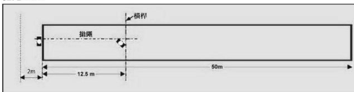
FIGURE 8: 拋繩12.5m
